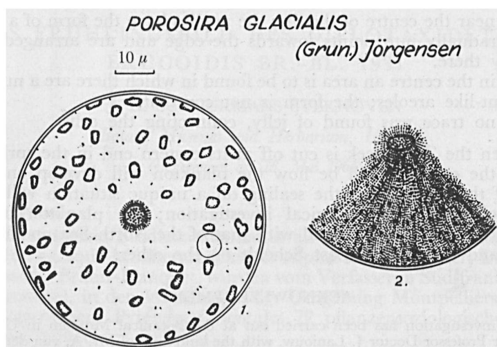
Fig. 3. Porosira glacialis (Grun.) Jörgensen. Part of the disc.
