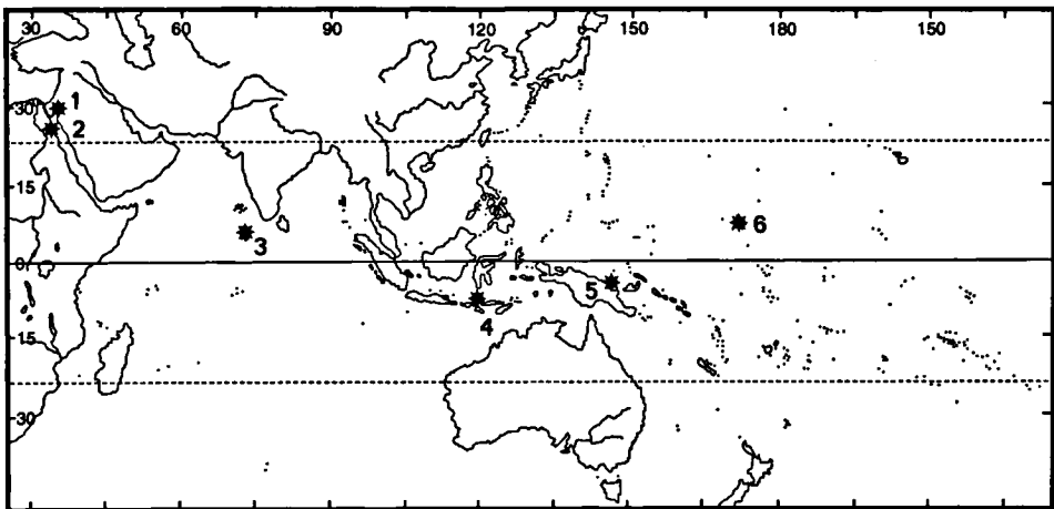
Fig. 13. The presently known range of Fungiacava eilatensis in the Indo-Pacific (references in table 1): 1. Gulf of Eilat (Israel and Egypt), 2. Safaga (Egypt), 3. Maldives, 4. Komodo Island (Indonesia), 5. Hansa Bay (N. Papua New Guinea), 6. Marshall Islands, exact locality unknown.
