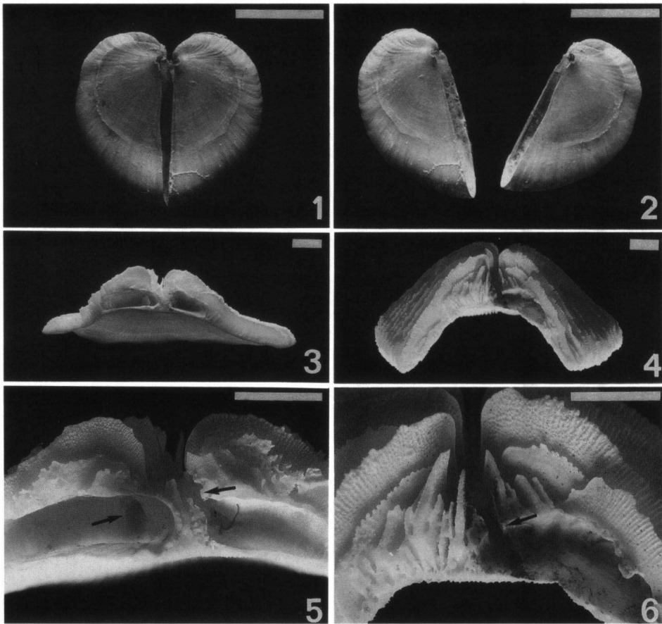
Figs. 1-6. Fungiacava eilatensis infesting Fungia (Cycloseris) fragilis ; specimens from Komodo Island, Indonesia (RMNH Coel. 21414); scale bars 0.5 cm. 1-2. A complete pair of empty shells (from the coral shown in figs. 3 and 5). The two host corals in cross-section showing the position of the cavities, one (3) with two cavities and another (4) with a single one. 5-6. The location of the siphon canals (arrows) in the same corals.
