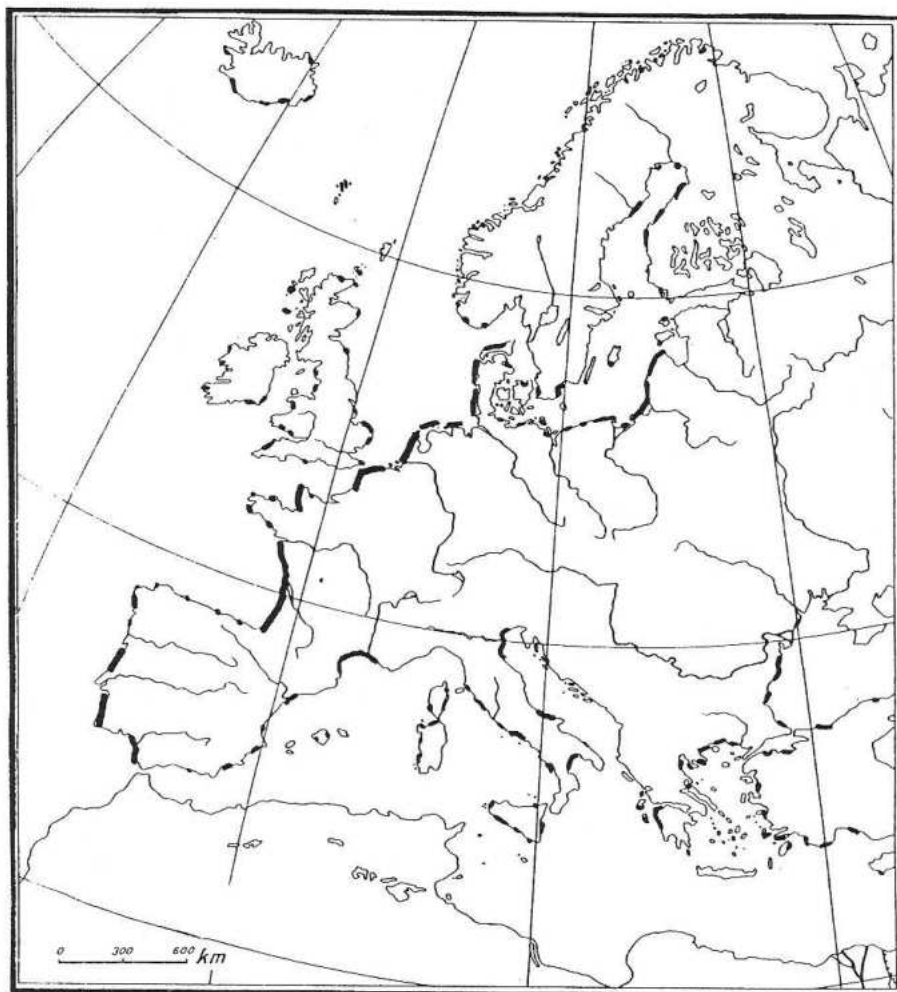
De belangrijkste duingebieden in Europa (uit: J.M. Gehu, 1985. European dune and shoreline vegetation . Nature and Environment Series 32, Council of Europe, Strasbourg).
