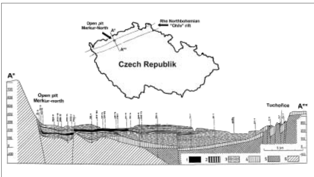
Figure 1 Geological cross section through the North Bohemian Ohre rift with the Tertiary browncoal basin. Cross section (line A*-A** in the map) through the North Bohemian Tertiary browncoal basin in the Chomutov-Most region, showing the asymmetrical shape of the Ohre rift caused by the volcano-tectonic subsidence (10x height exaggeration). 1 - the Miocene sequence (browncoal seams, humolitic clays and clay-stones); 2 - Lower Miocene freshwater limestones at Tuchorice and Lipno recorded in the partial tectonic relics (fault blocks) along the tectonic Krusné Hory Mountains and Ohre lines; 3 - Tertiary sands and clays; 4 - Upper Cretaceous sediments; 5 - Permocarboniferous sediments; 6 - metamorphic rocks of the Krusné Hory Mountains.
