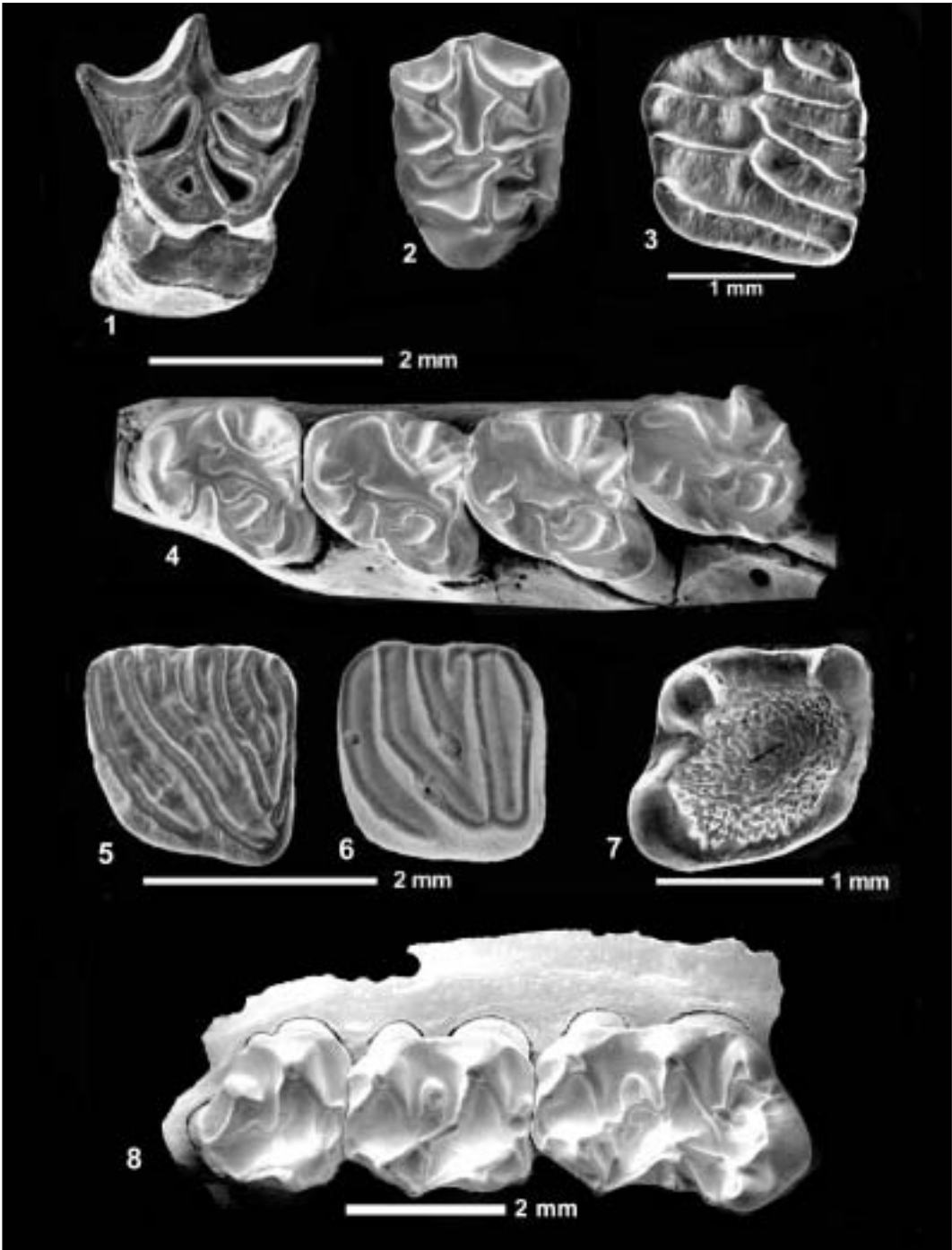
Plate 5. Examples of rodents from the base of the main brown coal seam from the open pit Merkur-North. 1, 2, 4 : the aplodontids: 1 : Ameniscormys selenoides DEHM, upper left M I, (an unique record from a deep drilling in 1964 in the area of the future open pit Merkur-North), 2, 4 : Plesispermophilus descendens DEHM, upper right M I (2) and lower left p4 - m3 in a mandible; 5, 6 : the gliroid Myoglis antecedens MAYR, upper left P 4 ( 5 ) and M I-2 ( 6 ); 7 : the small petauristid Blackia miocaenica MEIN, lower left m1-2; 8 : upper right maxilla (inverse) of the aberrant cricetid Melissiodon dominans DEHM, with M I-3.
