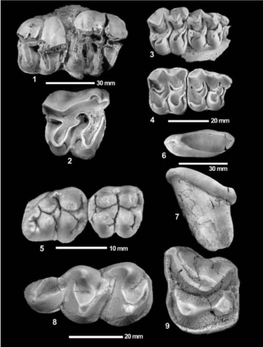
Plate I 1: Protaceratherium minutum (CUVIER), left upper P3, P4, occlusal; 2: Prosantorhinus n. sp., right upper M1 re., occlusal; 3, 4: Anchitherium aurelianense (CUVIER) upper right P3, P4, juvenile (3) and adult (4) individual; 5: Propalaeochoerus aurelianensis right upper M2, M3; 6, 7: 'Diaceratherium' douvillei (OSBORN), left upper incisor I 1, occlusal (6) and medial (7); 8, 9: Brachyodus onoides (DEPERET) right lower m3 (8) and right upper P2. 1, 2, 5 - 9: from Tuthorice travertine section "Reuss-Suess", 3, 4: from the base of the main coal seam, open pit Merkur-North. Occlusal (1 - 6, 8, 9) and medial (7) views.
