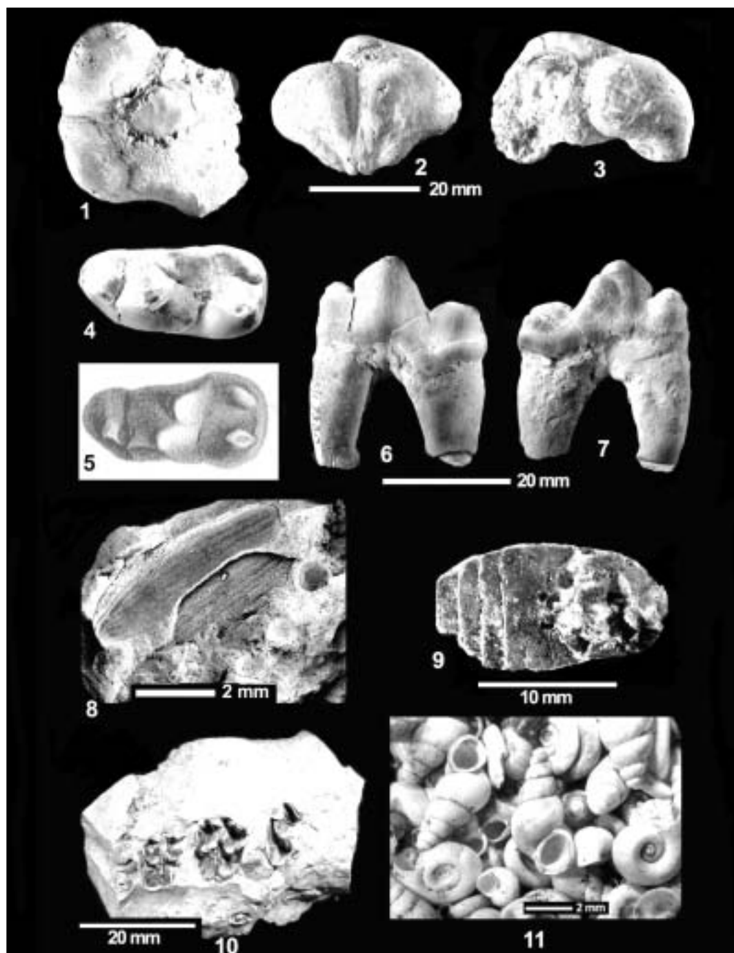
Plate 2 1 - 3 : Endocranial cast of a bird ( Accipitridae indet.), views: dorsal ( 1 ), frontal ( 2 ), lateral ( 3 ); 4 - 7 : Amphicyon bohemicus SCHLOSSER, the Type: lower left m I (coll. CU, No. 7330), views: occlusal ( 4 ), copy of the original figure 1861 ( 5 ), buccal ( 6 ), lingual ( 7 ); 8 - 9 : examples of the insects: impression of a wing-case in a calcified coprolite, Merkur-North ( 8 ), ventral view of an encrusted small beetle, travertine section of Tucherice ( 9 ); 10 : rare record of a small cervid ("enamel shells" of the dislocated upper molars of cf. Procervulus ) in the bedded freshwater limestone facies from Tucherice; 11 : rich small freshwater gastropods (the prevailing genus Nystia ) in the base of the brown coal seam in the open pit Merkur-North.
