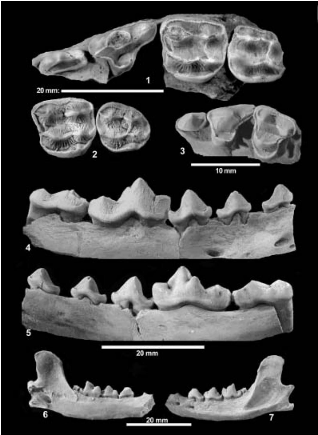
Plate 3 Examples of the carnivores from the base of the main brown coal seam from the open pit Merkur-North. 1, 2, 4, 5: Ballusia elmensis DEHM, upper left maxilla, P3 - M2 ( 1 ); 2: juvenile upper left M1-2; 4, 5: right mandible p1 - m1, views buccal ( 4 ) and lingual ( 5 ); 3: Stomeriella franconica DEHM, left maxilla P3 - M1; 6, 7: Palaeogale hyaenoides DEHM, left mandible p3 - m2.
