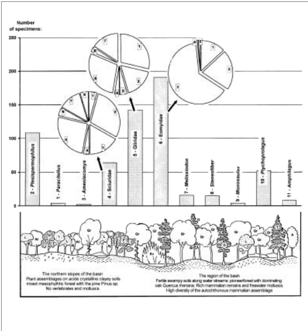
Figure 2 Above: Statistics of the frequency of the high diversified small mammalian assemblage in Merkur-North:
