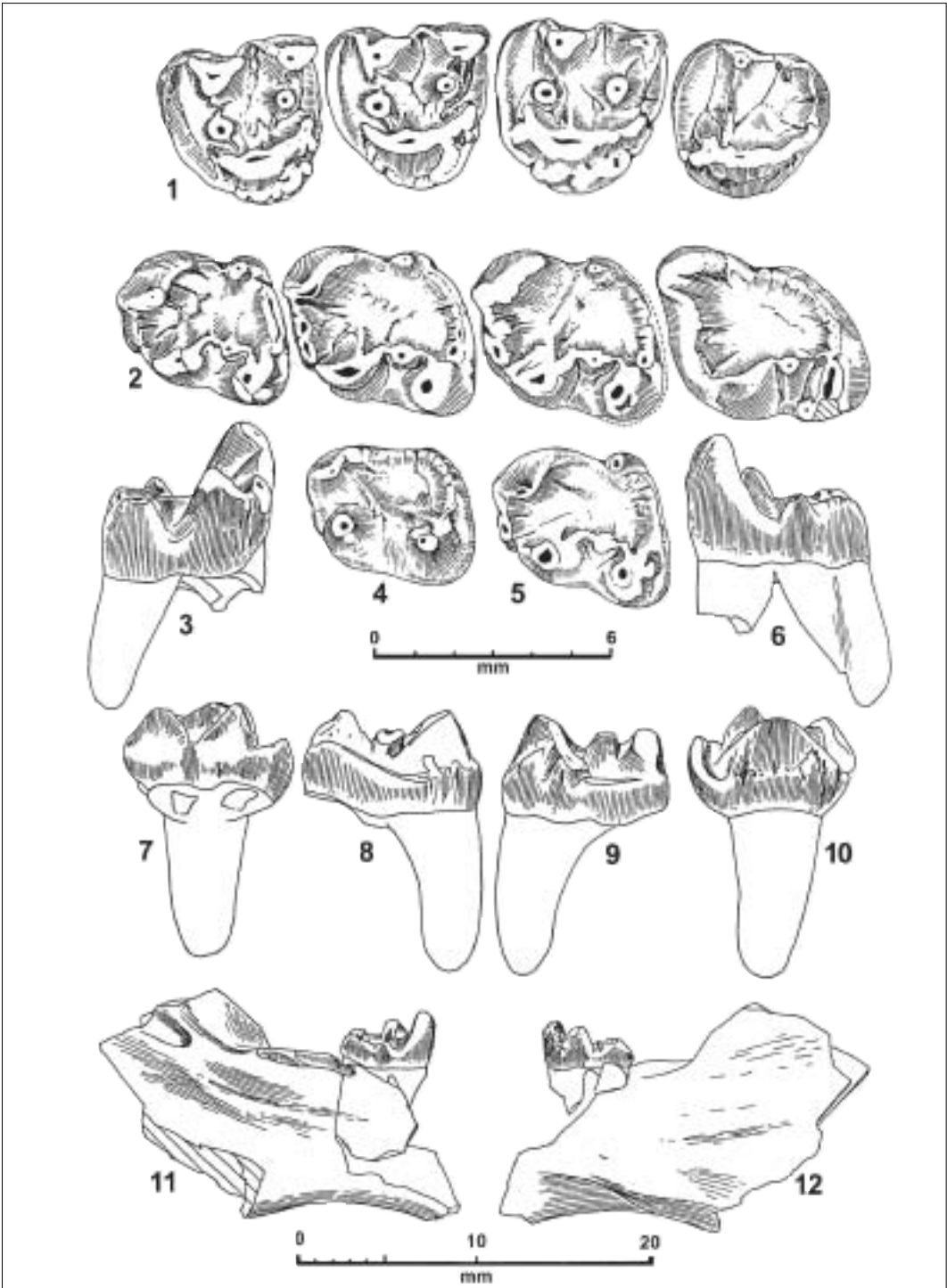
Figure 5. Paracitellus eminens ДЕМ, 1950 from Merkur-North. 1 - Upper left P4 - M3; 2 - lower left p4 - m3; 3, 5, 6 - lower m1, buccal ( 3 ), occlusal ( 5 ) and lingual ( 6 ) views; 4 - left deciduous Dp; 7 - 10 : upper M2 buccal ( 7 ), mesial ( 8 ), distal ( 9 ) and lingual ( 10 ) views; 11, 12 : fragment of the left lower jaw with m2 in situ. Collection of Z. Dvůrák.
