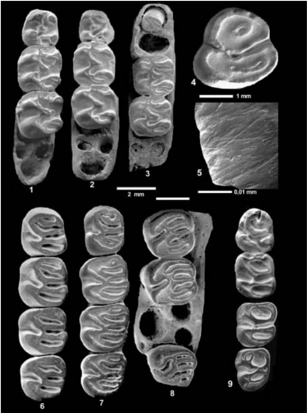
Plate 4 Examples of eomyids from the base of the main brown coal seam from the open pit Merkur-North. 1 - 3: Bunodont genus Pentabuneomys represented by two (?) forms sp. I and II, 4, 5: the giant Megapeomys lavocati FEJFAR et al., lower left p4 occlusal ( 4 ), detail of the scratched occlusal surface of enamel (prove of the fossorial habit of this species ?); 6 - 9: Lophodont genera Pseudotheridomys sp. ( 6 - 8 ) and Ligerimys lophidens DEHM ( 9 ).
