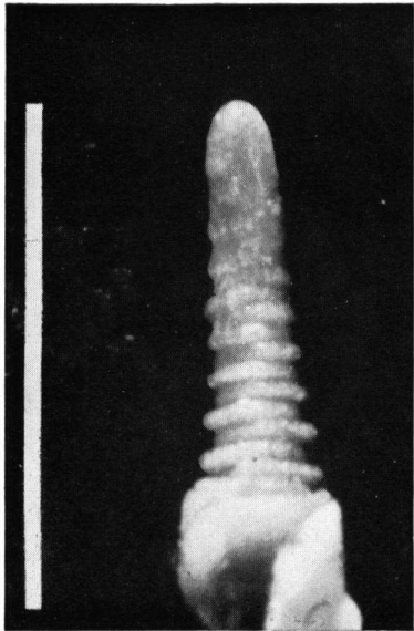
Vegetative apex
