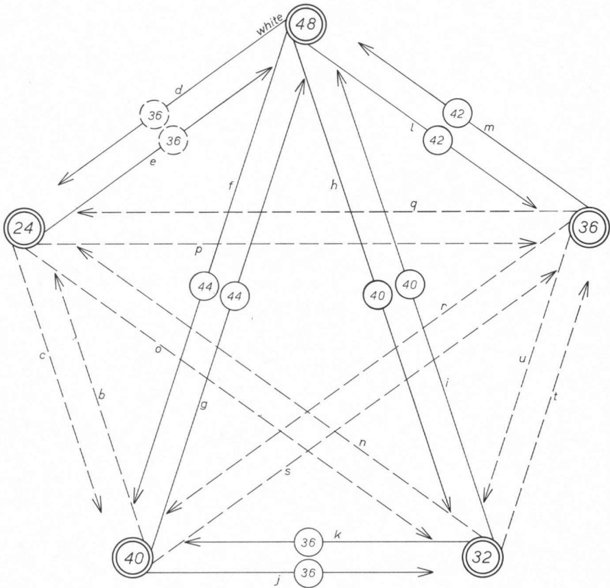
Fig. 1. Crossing-polygon, showing the relationships between Symphytum asperum Lepech. and Symphytum officinale L.
