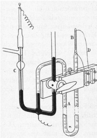
Figur 1. Toluolthermoregulator.
