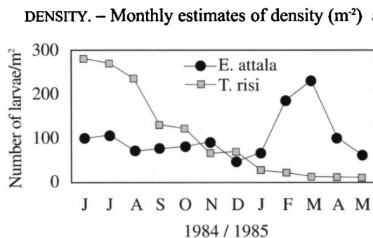
Fig. 2. Density of Erythemis attala and Tauriphila risi larvae from June 1984 to May 1985.
