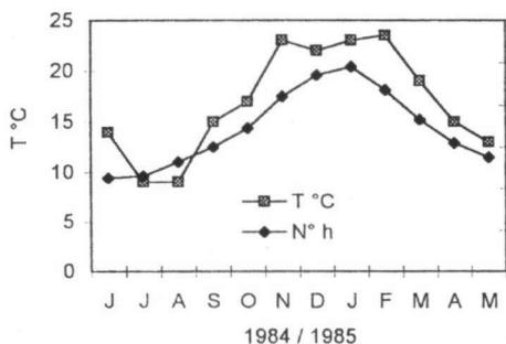
Fig. 1. Temperature of water sampling and number of effective hours of sunlight from June 1984 to May 1985. The values of effective sunlight are based on data from the Observatory of La Plata from 1961 to 1970.
