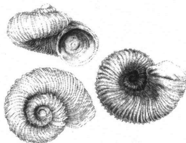
Maizaniella falkneri - De Winter, 2002, Collectanea Malacologica: fig. 2
