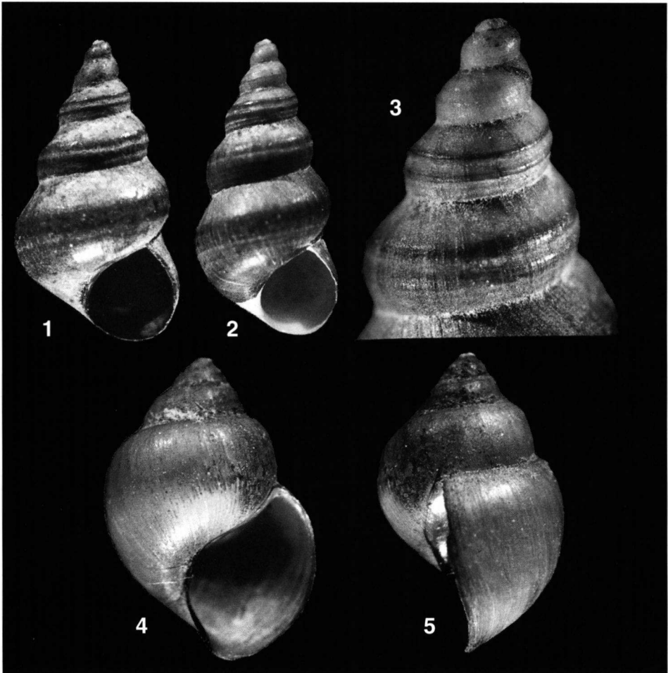
Figs 1-5. Hydrobiid species. 1-3, Dyrus amazonicus Haas, 1949; paratypes (FMNH 29198); Recent, Tapajos river, Belterra, Para, Brazil (1, H 5.0 mm; 2, H 6.4 mm; 3, detail of 2). 4-5, Sioliella effusa Haas, 1949, holotype (FMNH 29209); Recent, Tapajos river, Belterra, Para, Brazil; H 6.4 mm.
